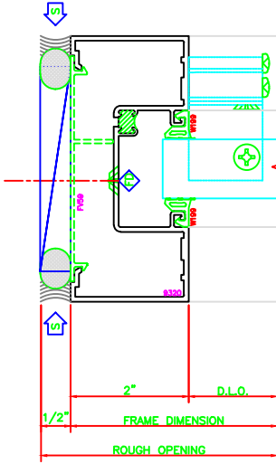
402 JAMB 403 SHEARBLOCK
